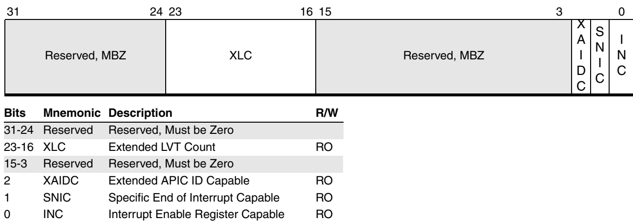
Figure 16-28. Extended APIC Feature Register (APIC Offset 400h)
