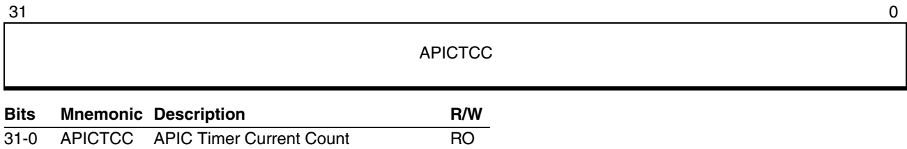
Figure 16-8. Timer Current Count Register (APIC Offset 390h)
