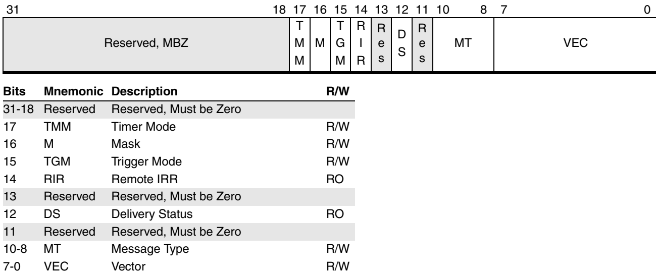
Figure 16-6. General Local Vector Table Register Format
