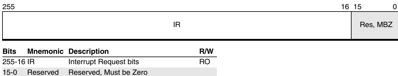
Figure 16-22. Interrupt Request Register (APIC Offset 270:200h)
