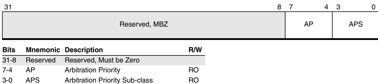
Figure 16-21. Arbitration Priority Register (APIC Offset 90h)
