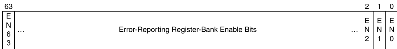
Figure 9-3. MCG_CTL Register
