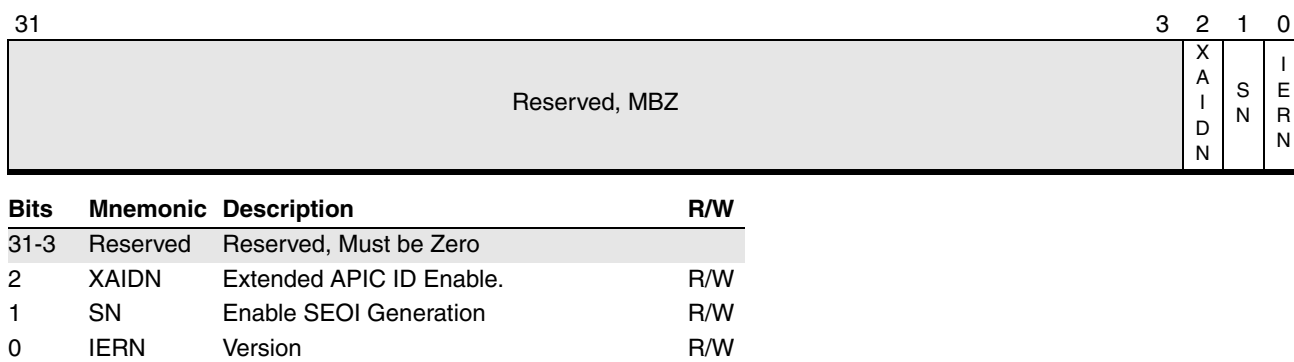
Figure 16-5. Extended APIC Control Register (APIC Offset 410h)
