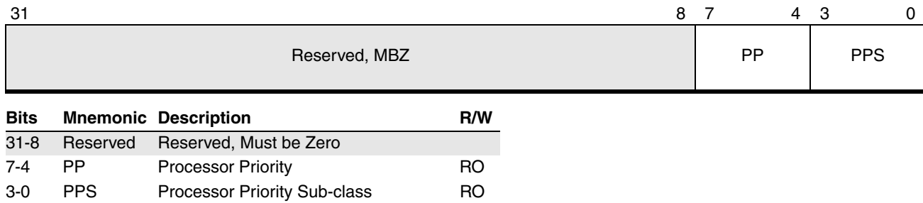
Figure 16-26. Processor Priority Register (APIC Offset A0h)
