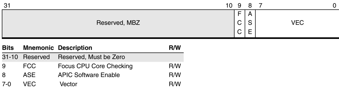
Figure 16-16. Spurious Interrupt Register (APIC Offset F0h)
