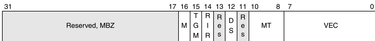
Figure 16-11. Local Interrupt 0/1 (LINT0/1) Local Vector Table Register (APIC Offset 350h/360h)
