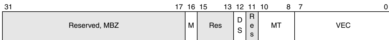
Figure 16-14. APIC Error Local Vector Table Register (APIC Offset 370h)
