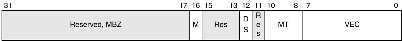
Figure 16-12. Performance Monitor Counter Local Vector Table Register (APIC Offset 340h)
