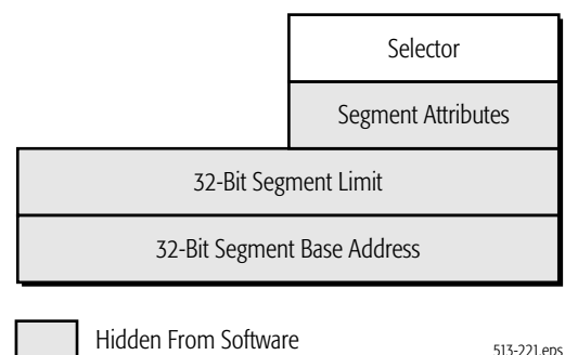
Figure 4-4. Segment-Register Format
