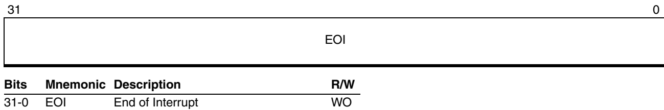
Figure 16-27. End of Interrupt (APIC Offset B0h)
