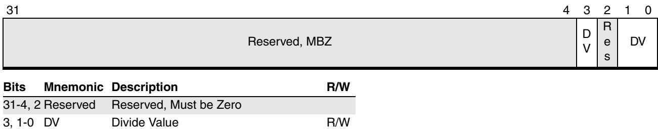
Figure 16-10. Divide Configuration Register (APIC Offset 3E0h)
