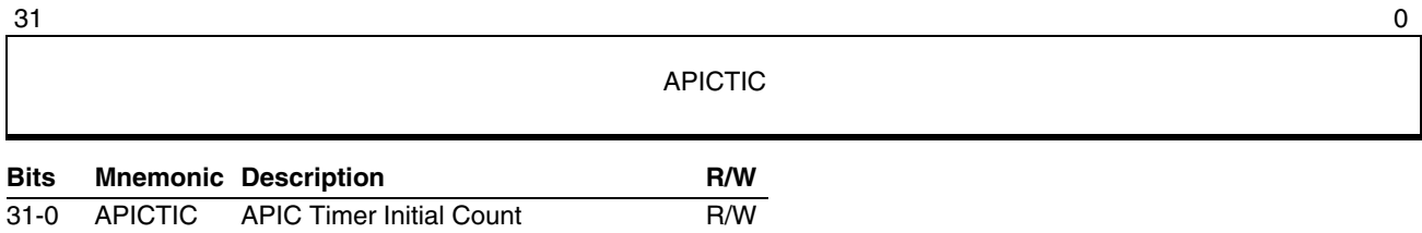
Figure 16-9. Timer Initial Count Register (APIC Offset 380h)
