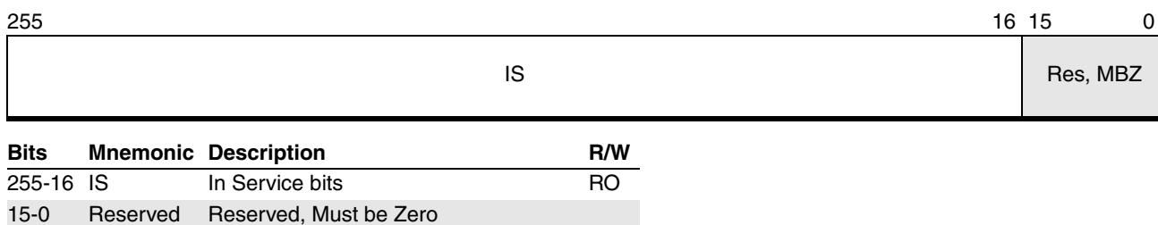
Figure 16-23. In Service Register (APIC Offset 170:100h)
