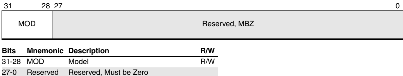
Figure 16-20. Destination Format Register (APIC Offset E0h)
