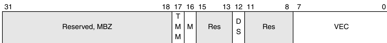
Figure 16-7. APIC Timer Local Vector Table Register (APIC Offset 320h)
