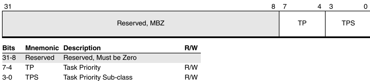
Figure 16-25. Task Priority Register (APIC Offset 80h)
